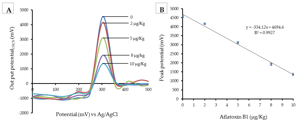
Figure 1. (A) DSCV signal recorded for HRP-blocked immune-electrode for different aflatoxin B 1 concentrations (0–10 \mu\text{g/kg} ) in a citrate buffer pH 7.0 (scan from 0 to 500 mV; pulse amplitude 56 mV; pulse width 460 ms, and scan rate of 20 mV/s). (B) A calibration curve of peak DSCV potential (mV) versus aflatoxin B 1 concentration ( \mu\text{g/kg} ).
